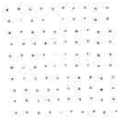
very fine
