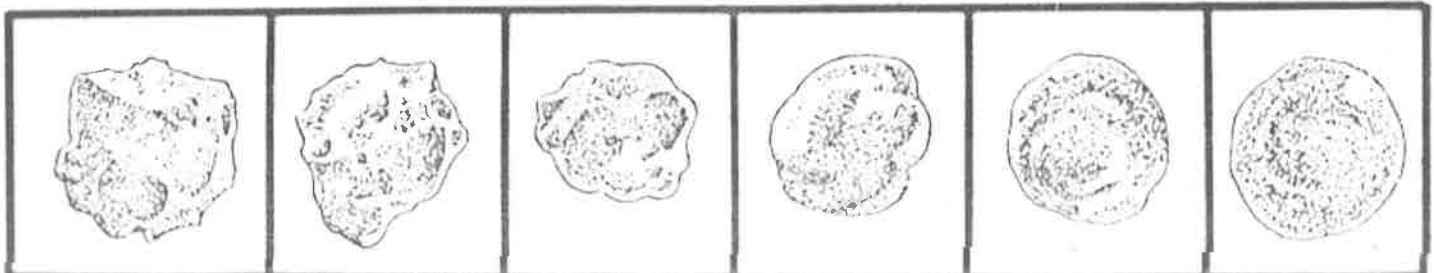
SUB ANGULAR
