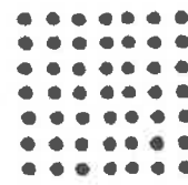
coarse
