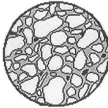
Well Sorted
