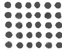
very coarse
