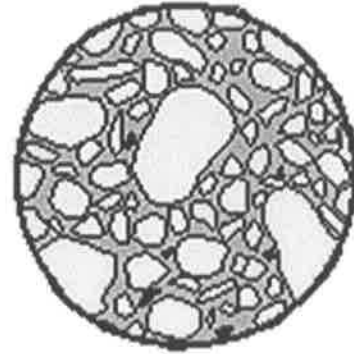
Moderately Sorted
